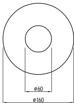
TOPPVY 1 : 5
