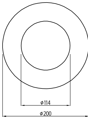
TOPPVY 1 : 5
