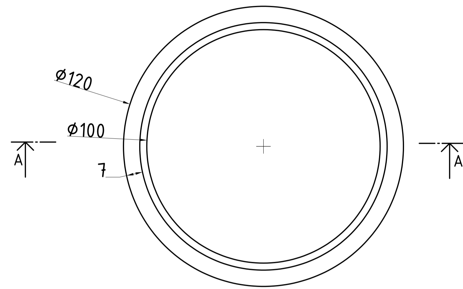
TOPPVY 1:1
