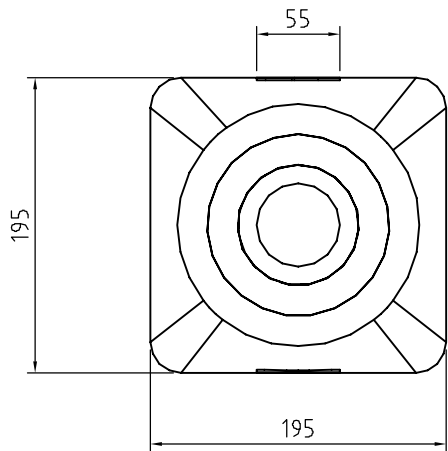
TOPPVY 1:5
